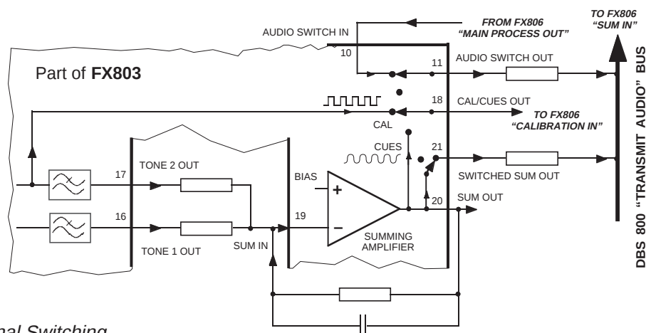
Fig.3 Output Signal Switching
