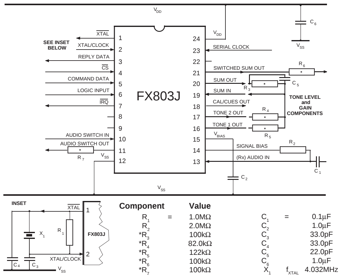
Fig.2 Recommended External Components
