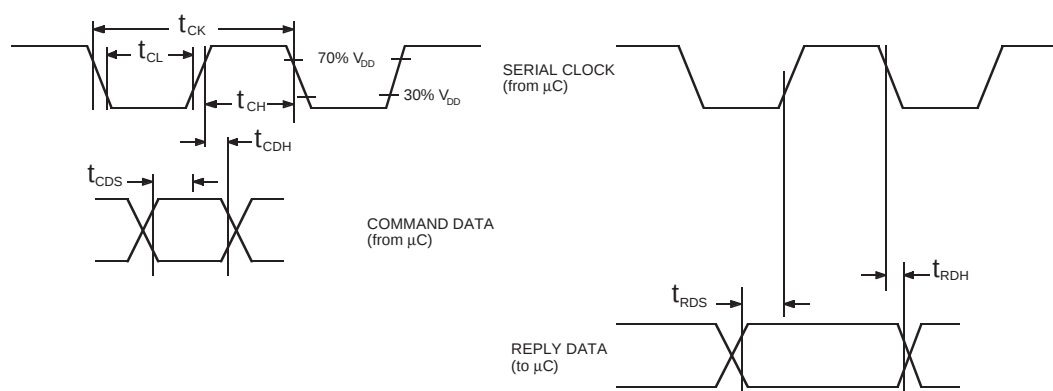
Fig.8 "C-BUS" Timing Relationships
