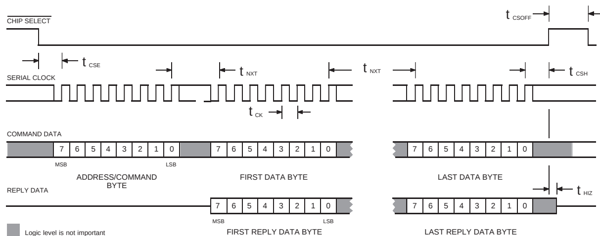
Fig.7 "C-BUS" Timing Information
