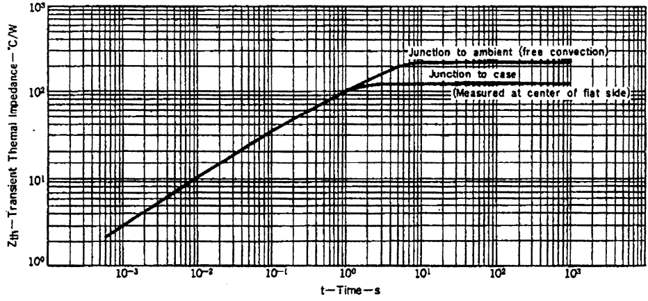
Fig. 12 Z_{th} CHARACTERISTICS
