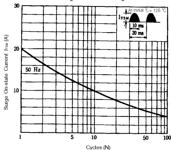
Figure 2. I_{TSM} Rating
