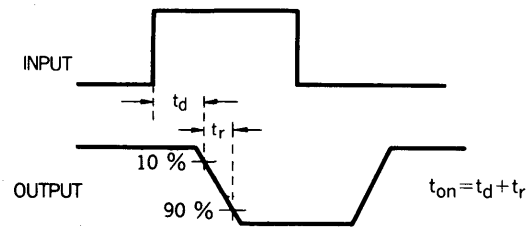
VOLTAGE WAVEFORMS
