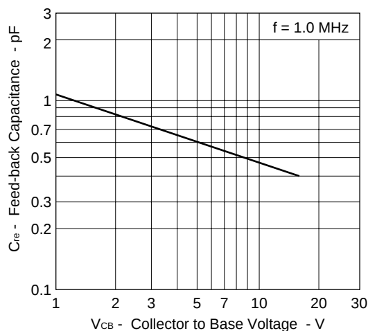
TYPICAL DEVICE CAPACITANCE vs. COLLECTOR TO BASE VOLTAGE
