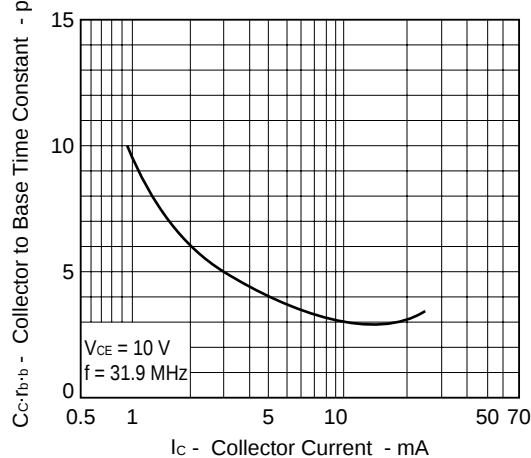
COLLECTOR TO BASE TIME CONSTANT vs. COLLECTOR CURRENT
