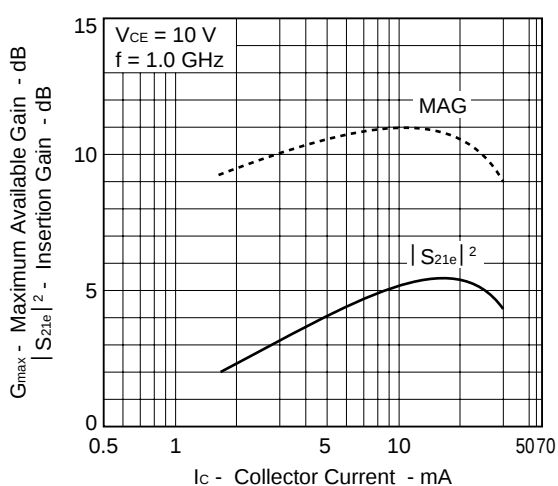
INSERTION GAIN, MAXIMUM AVAILABLE GAIN vs. COLLECTOR CURRENT
