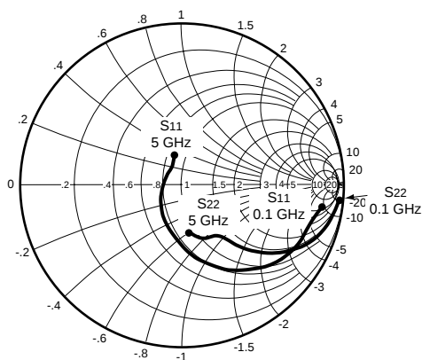
Coordinates in Ohms Frequency in GHz ( V_{CE} = 2\text{ V} , I_C = 3\text{ mA} )
