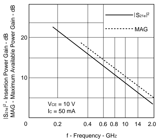
INSERTION POWER GAIN MAXIMUM AVAILABLE GAIN vs. FREQUENCY
