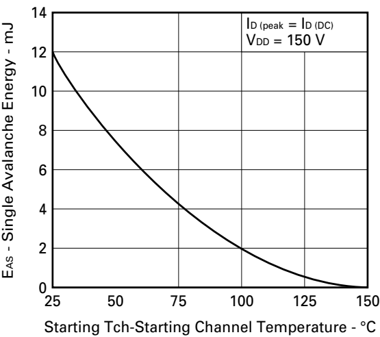
SINGLE AVALANCHE ENERGY vs. STARTING CHANNEL TEMPERATURE
