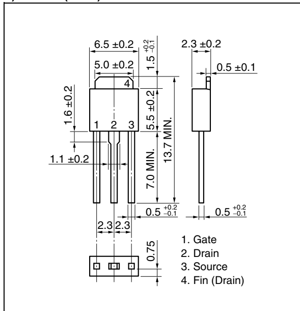
1) TO-251 (MP-3)
