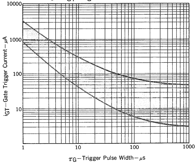
Fig. 7 I_{GT} - \tau_G TYPICAL DISTRIBUTION
