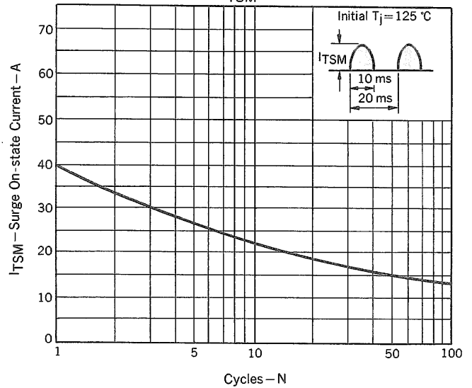
Fig. 2 I_{TSM} RATING
