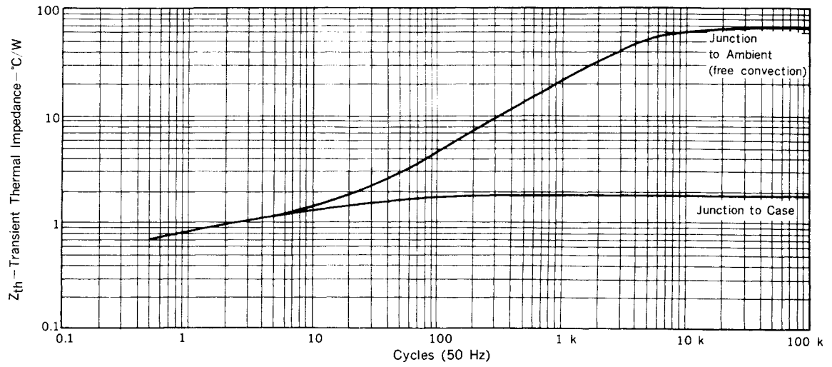
Fig. 13 Z_{th} CHARACTERISTIC
