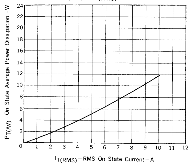
Fig. 10 P_{T(AV)} - I_T(\text{RMS}) CHARACTERISTIC
