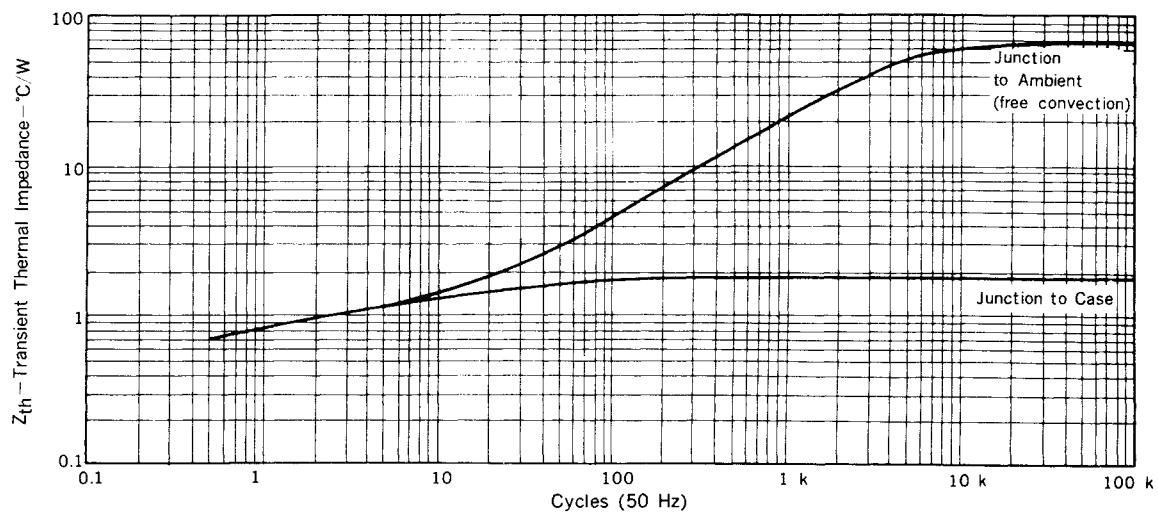
Fig. 13 Z_{th} CHARACTERISTIC
