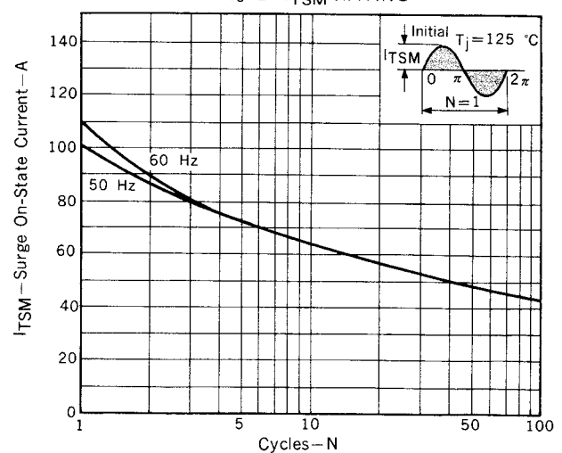
Fig. 2 I_{\text{TSM}} RATING
