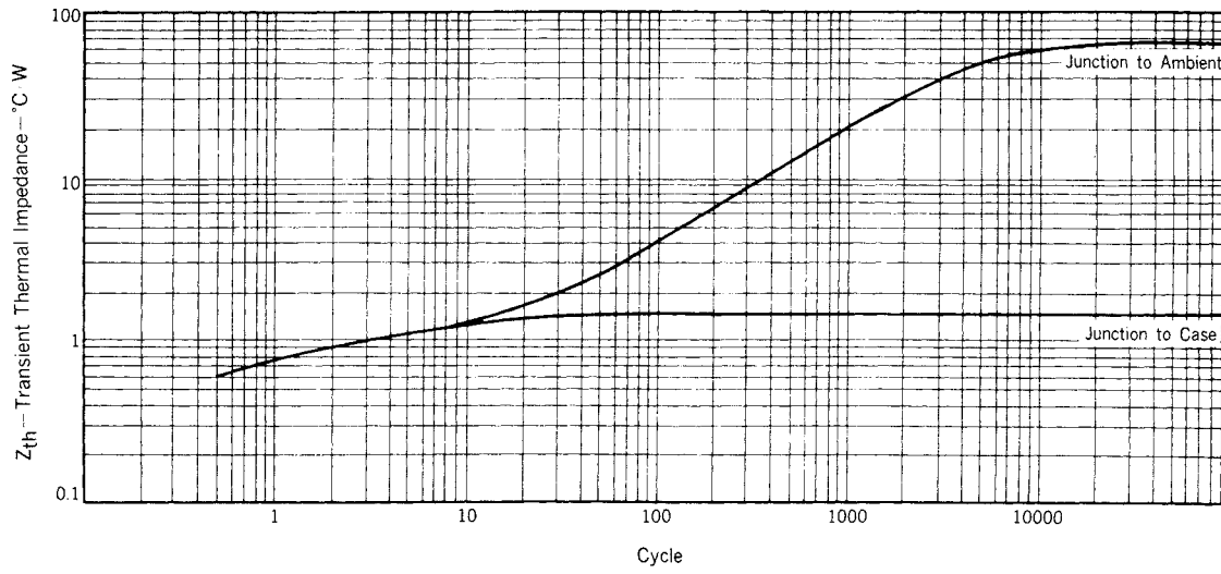
Fig. 13 Z_{th} CHARACTERISTIC
