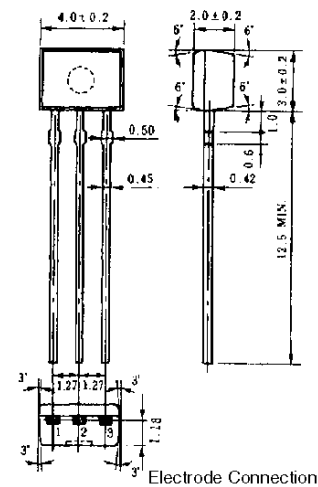
Electrode Connection
