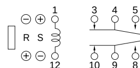
Single coil latch type (reset position)
