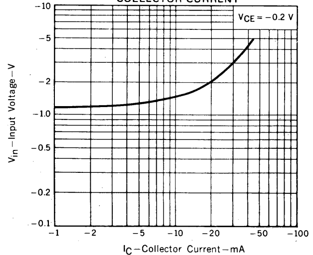
INPUT VOLTAGE vs. COLLECTOR CURRENT
