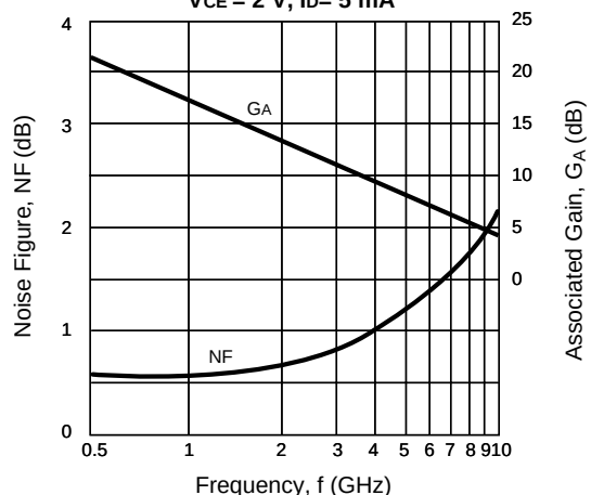
NOISE FIGURE & ASSOCIATED GAIN vs. FREQUENCY V CE = 2 V, I D = 5 mA
