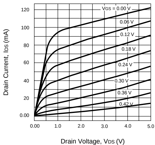
DC PERFORMANCE
