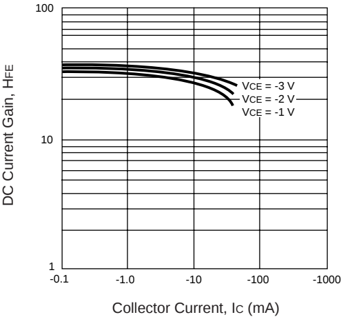
DC CURRENT GAINS vs. COLLECTOR CURRENT
