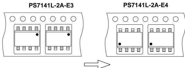
TAPING DIRECTION
