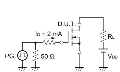
TEST CIRCUIT 2 GATE CHARGE
