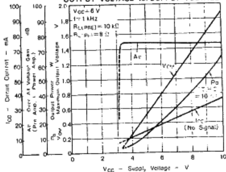
CIRCUIT CURRENT, OVER ALL VOLTAGE GAIN, OUTPUT POWER, MAXIMUM OUTPUT VOLTAGE vs. SUPPLY VOLTAGE
