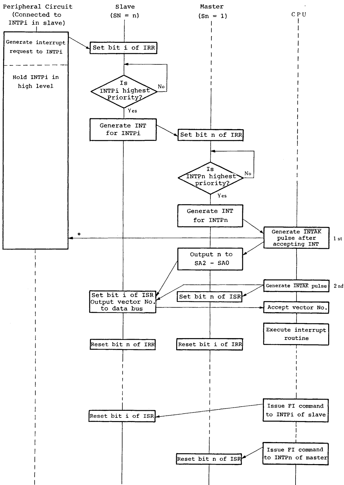
Fig. 5-5 Interrupt from Slave (Vector Mode)
