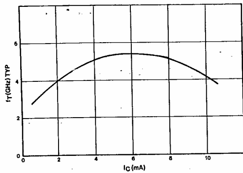
Fig. 2 Collector current
