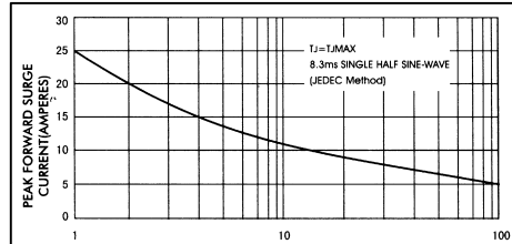
FIG.2-MAXIMUM NON-REPETITIVE PEAK FORWARD SURGE CURRENT
