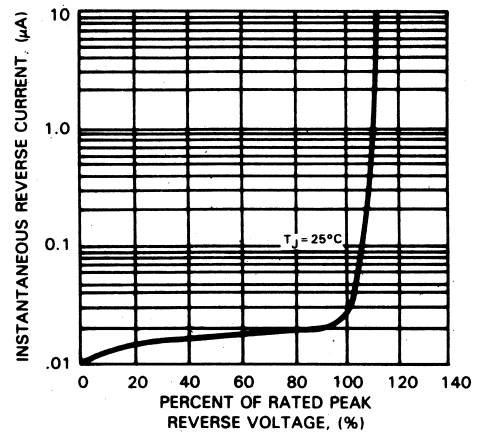
FIG.4-TYPICAL REVERSE CHARACTERISTICS
