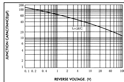
FIG.4-TYPICAL JUNCTION CAPACITANCE
