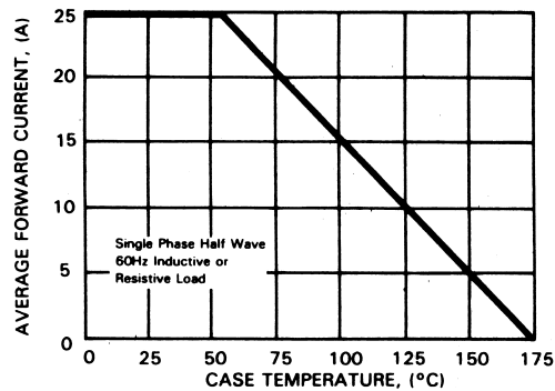
FIG.2-TYPICAL FORWARD CURRENT
