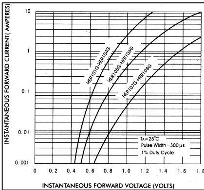
FIG.3-TYPICAL FORWARD CHARACTERISTICS
