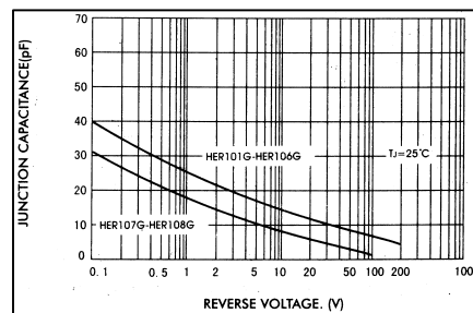
FIG.6-TYPICAL JUNCTION CAPACITANCE
