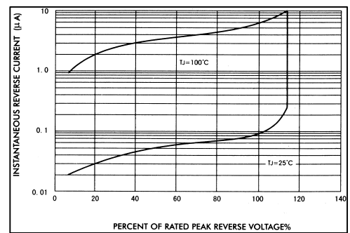
FIG.4-TYPICAL REVERSE CHARACTERISTICS
