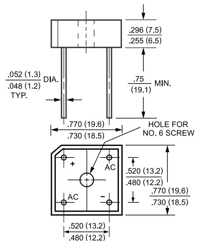
KBPC-8/10
