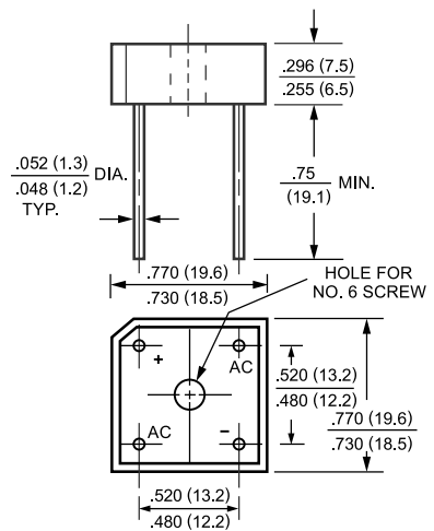
KBPC-8/10
