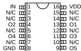
3D7205S SOIC (300 Mil)
