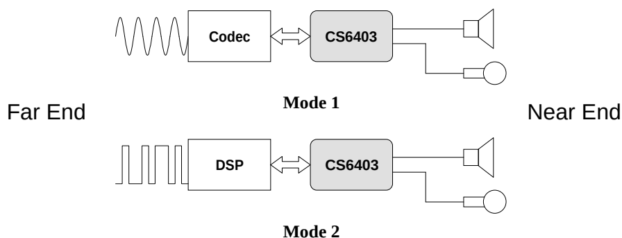
Figure 4. Operating Modes
