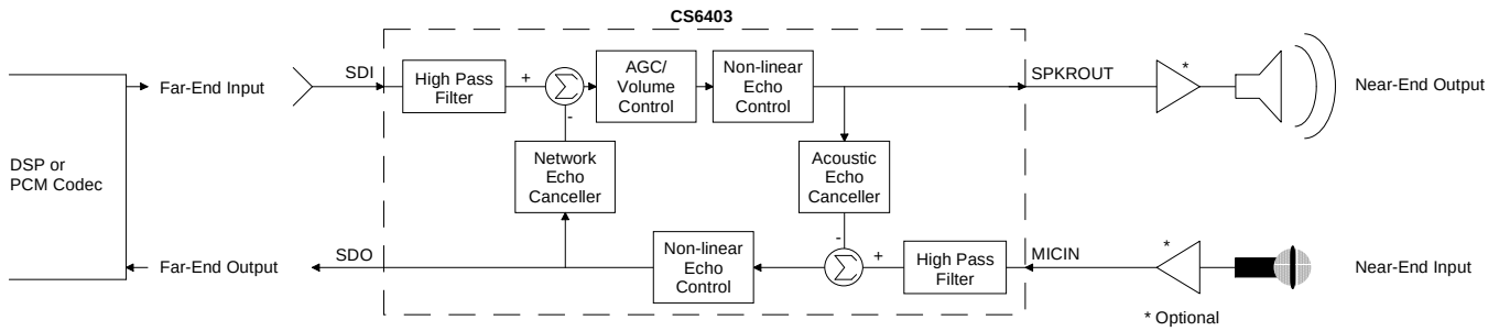
Figure 3. Functional Diagram
