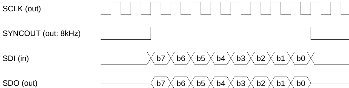
Figure 6. External-Codec Mode Timing (Mode 1)
