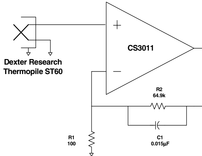
Figure 13. Thermopile Amplifier with a Gain of 650 V/V
