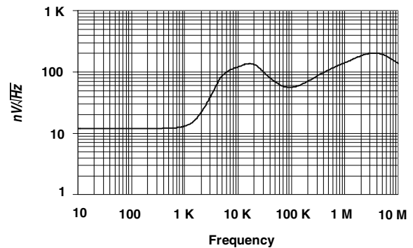
Figure 3. Noise vs Frequency
