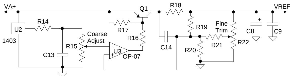
Figure 3. Voltage Reference Circuitry
