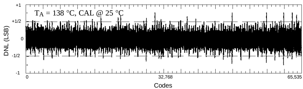
Figure 12. CS5101A DNL Plot; Ambient Temperature at 138°C
