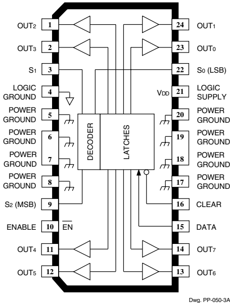
A6A259KLB (SOIC)
