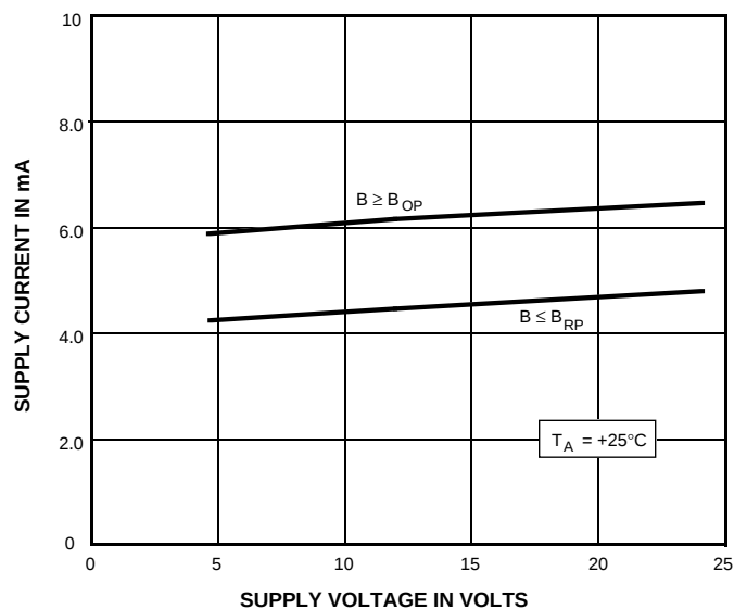
SUPPLY CURRENT
