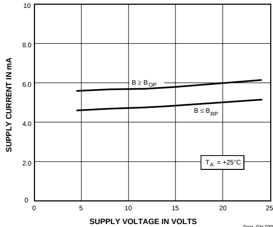
SUPPLY CURRENT
