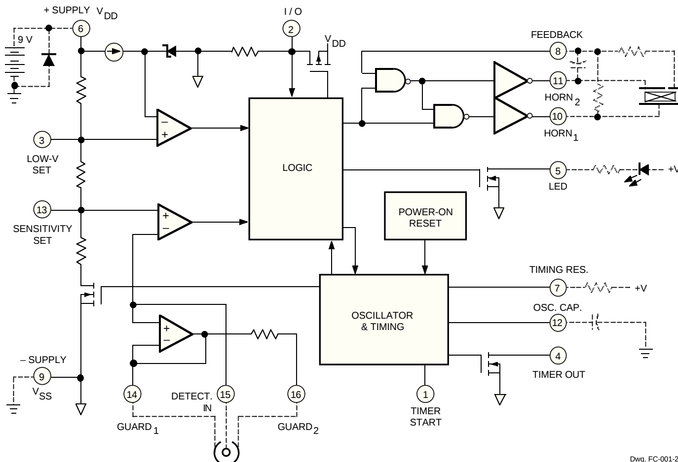
FUNCTIONAL BLOCK DIAGRAM AND TYPICAL APPLICATION
