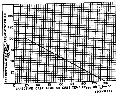
Fig. 2 - Current derating curve for all types.
