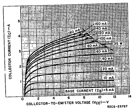
Fig. 15 - Typical output characteristics for 2N6500.
