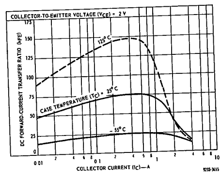
Fig. 14 - Typical dc beta characteristics for 2N5202.
