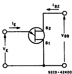
Fig. 1—Unijunction transistor symbol and nomenclature used for current and voltage circuit.
