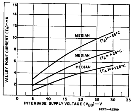
Fig. 7—Typical valley point current characteristic.
