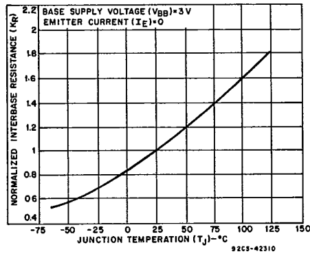
Fig. 8—Normalized interbase resistance characteristic.
