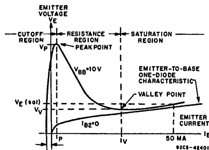
Fig. 3—Static emitter characteristics waveforms.
