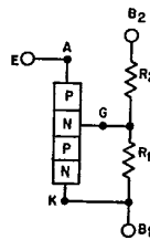
Programmable unijunction transistor equivalent circuit
