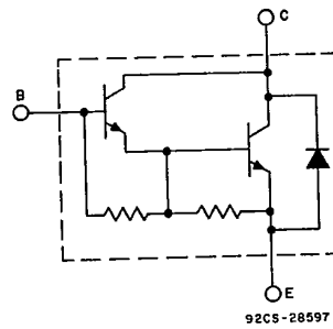
Fig. 1 — Schematic diagram for all types.
