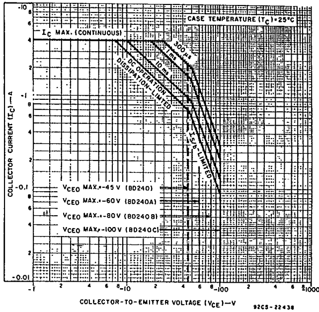
Fig. 1— Maximum safe operating areas for all types.
