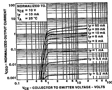
4. OUTPUT CHARACTERISTICS
