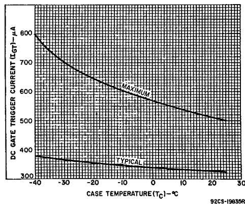
Fig. 10 — DC gate trigger current vs. case temperature for S2061 series.
