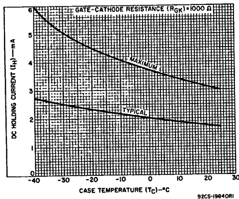
Fig. 13 — DC holding current vs. case temperature for the S2060 series.
