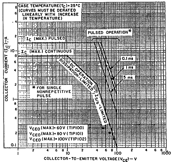
Fig. 4 - Maximum operating areas for all types ( T_C = 25^\circ\text{C} ).
