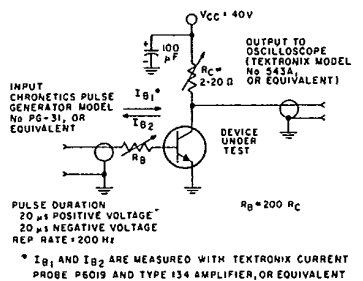
Fig. 5 - Circuit used to measure saturated switching times.
